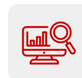
Log Monitoring
